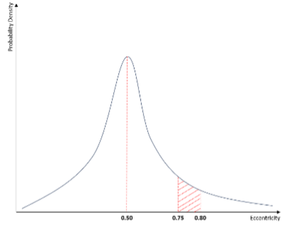
Figure 14: Probability distribution function (in blue) for eccentricity.
